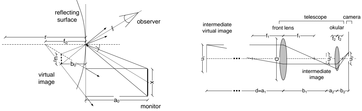
Figure 3. Size and location of the reflected image. The curvature of the sphere in the left part of the figure is exaggerated for illustration.
